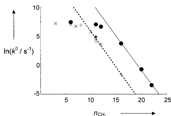
Figure 2. Plot of k^0 versus number of methylene groups for cytochrome c on SAM-coated gold electrodes ( \times from ref. [2c,d], + from ref. [2a,b], and \bullet from this work for COOH and \circ for pyridine-terminated layers). The lines are fits to Equation (1).
